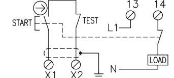
Monitoring to ensure that the On button is not stuck in pressed position. A short circuit over the closing contact is not monitored. The JSBR4 has built in short circuit monitored resetting.
